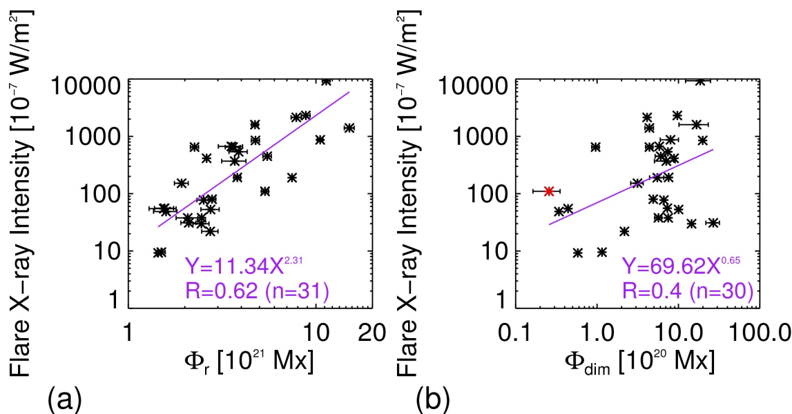
Figure 2. Scatter plot between (a) RC flux/poloidal flux and the soft X-ray flare size and (b) Dimming flux/toroidal flux and the soft X-ray flare size. The violet line is the regression of the data set. The correlation coefficients ( r ) and the number of data points ( n ) are shown on the plots. In the RC flux - flare size correlation, the correlation coefficient ( cc ) is within the 95% confidence interval (0.34,0.79); in the Dimming flux - flare size correlation, cc is within the 95% confidence interval (0.047,0.664). The cc obtained are significant. Outliers are shown in red.
