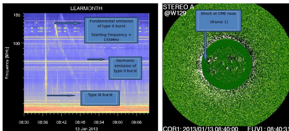
Figure 1. The left side is the 13 January 2013 type II burst observed by Learmonth solar radio spectrometer. As observed in figure 1(left), there is a fundamental harmonic structure of type II burst, which followed a type III burst. The starting frequency of the fundamental emission is 155 MHz. Figure 1 on the right shows the CME shock associated with the January 13, 2013 burst, it was observed two minutes after the appearance of type II.
