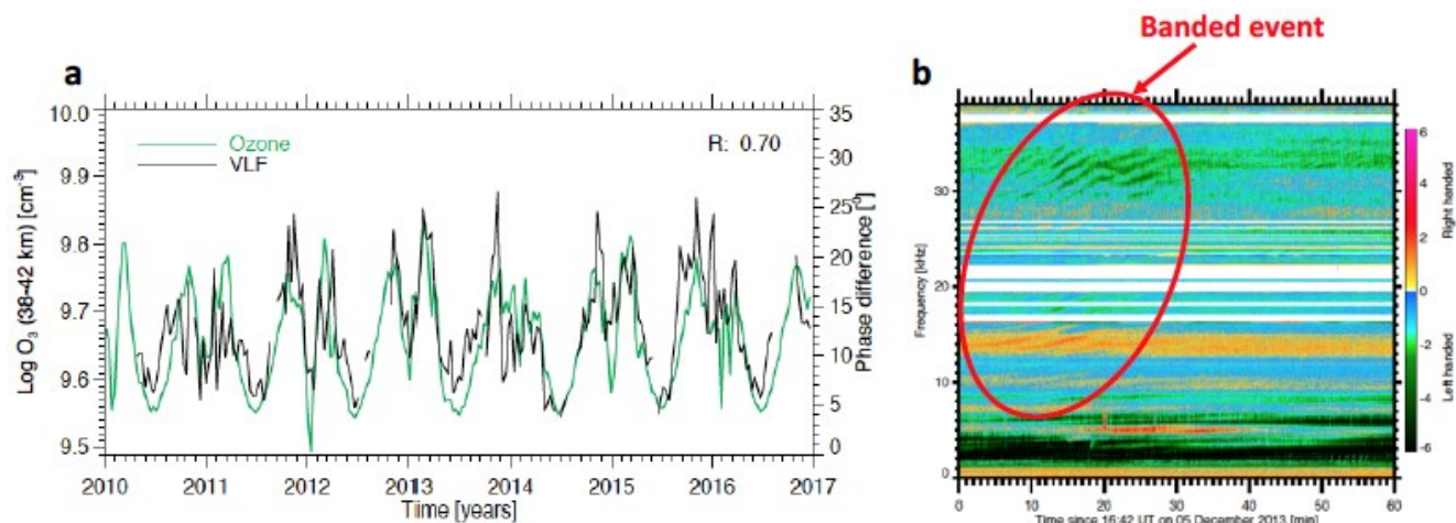
Figure 2. (a) 10-day averages of the amplitude phase perturbation variability (black curve) contrasted with the atmospheric ozone number density (green curve) at 38–42 km. R is the correlation coefficient. (b) Example of banded emission (within the red ellipse) observed at Kannuslehto. One-hour frequency-time spectrogram of right-handed (reddish colors) and left-handed (greenish colors) polarization ratio. Measurements on 05 December 2013 since 16:42 UT.
