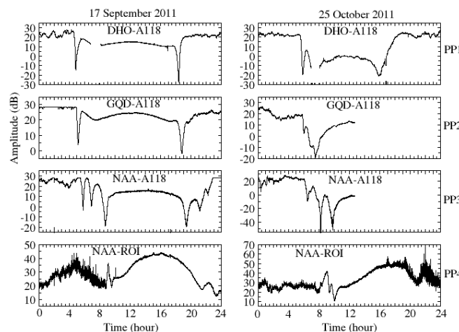
Figure 2. VLF signal anomaly observed in NAA-ROI propagation path during geomagnetic storms of 17 Sept. and 25 Oct. 2011.
