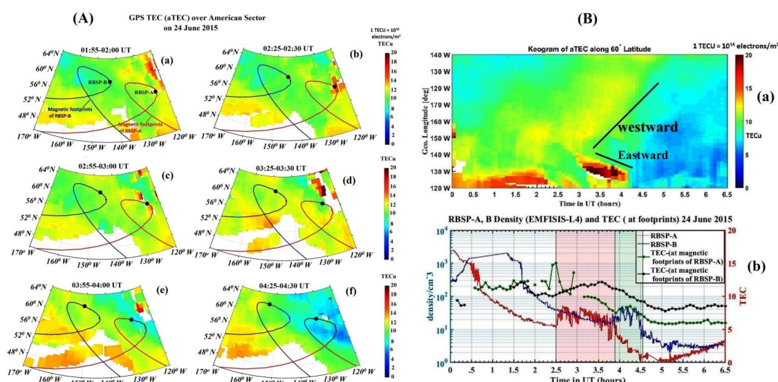
Figure 1. (A) shows the snapshots of GPS TEC between ~02:00-04:30 UT (~0.5 hr intervals) over the North American Sector on the 24 th June 2015. The blue and red curves show magnetic footprints of RBSP-A and B (~300 km). The electron density enhancement and longitudinal (westward) propagation depicts in figure A (a-c). The keogram of absolute TEC (aTEC) along the 60° latitude shows westward and eastward propagation of the electron density in the ionosphere (in the figure-B (a)). The bottom panel of the figure-B (b) shows, electron density variations obtained from the RBSP-A (red) and RBSP-B (blue). The green and black color curves show electron density variation at the magnetic footprints of RBSP-A and B in the ionosphere at ~300 km.
